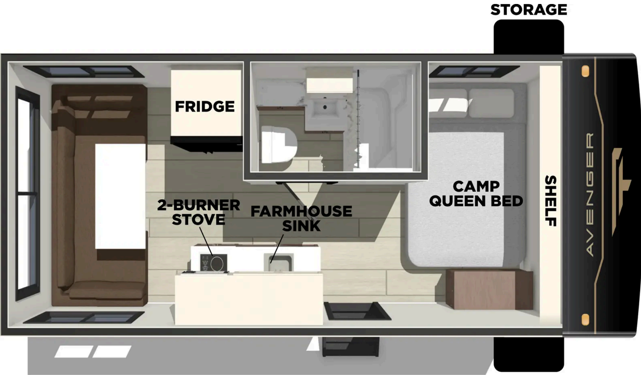
16RD FLOORPLAN
